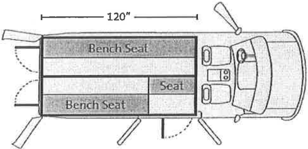
Prisoner Transport Insert For 2015-2016 Ford Transit Medium roof long length 148" wheel base cargo van Image 1 of 4
